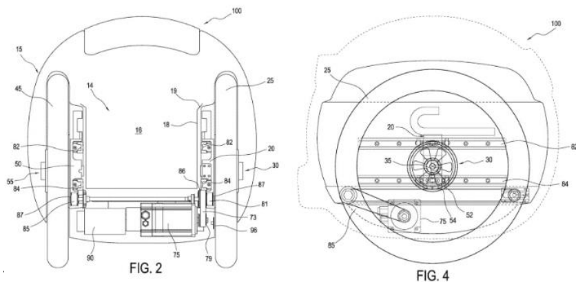
Drone terrestre, 2022
